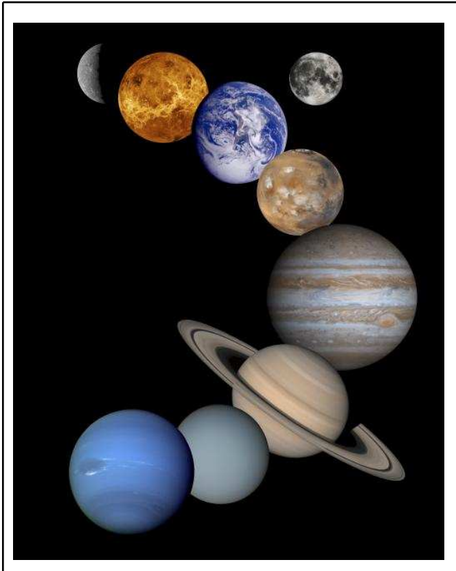
planets
